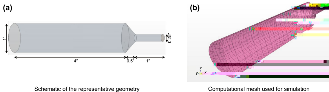
Fig. 10 Geometry of the computational domain: pipe with a restriction at the end
